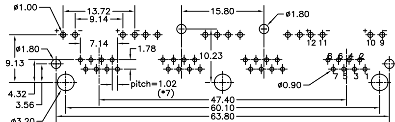
PC Board Layout(t=1.60mm) Component Side Shown Tolerance±0.05mm
