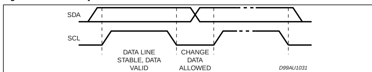
Figure 16. Data Validity on the I 2 C BUS
