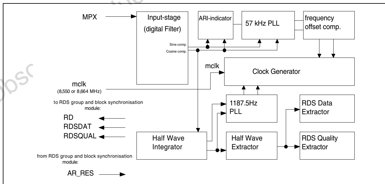
Figure 8. Demodulator Block Diagram
