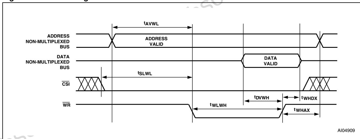
Figure 35. Write Timing
