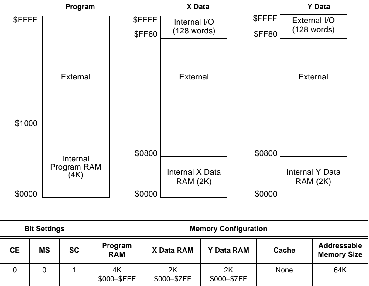
Figure 3-2. 16-Bit Space With Default RAM (0, 0, 1)
