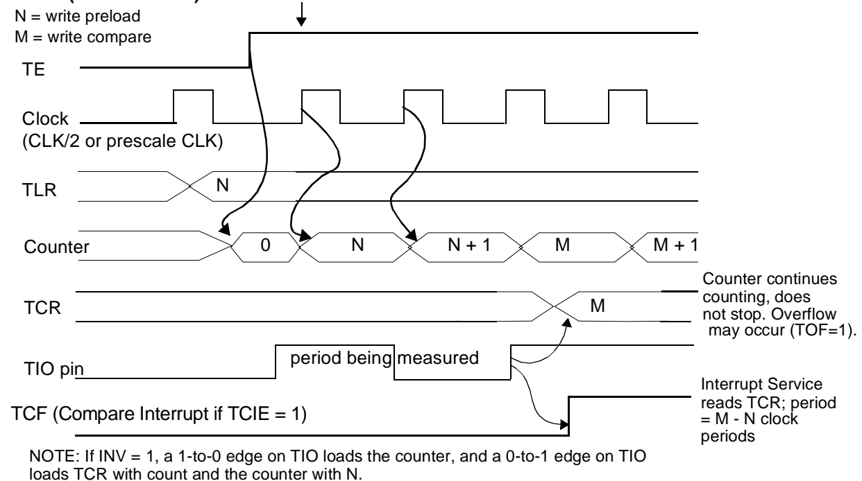
Figure 9-14. Period Measurement Mode, TRM = 0
