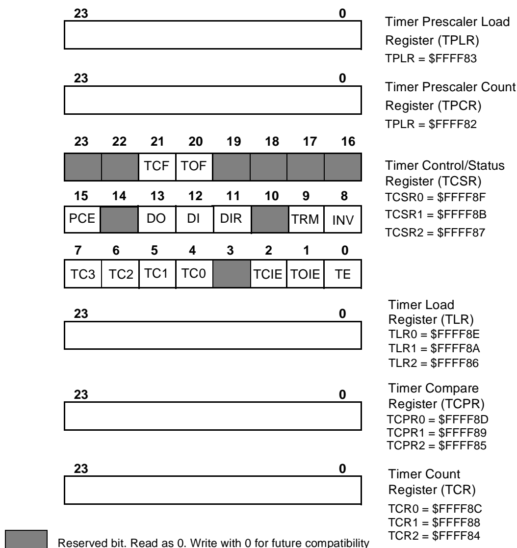
Figure 9-20. Timer Module Programmer's Model
