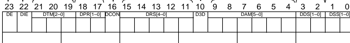
Figure B-9. DMA Control Registers 5–0 (DCR[5–0])
