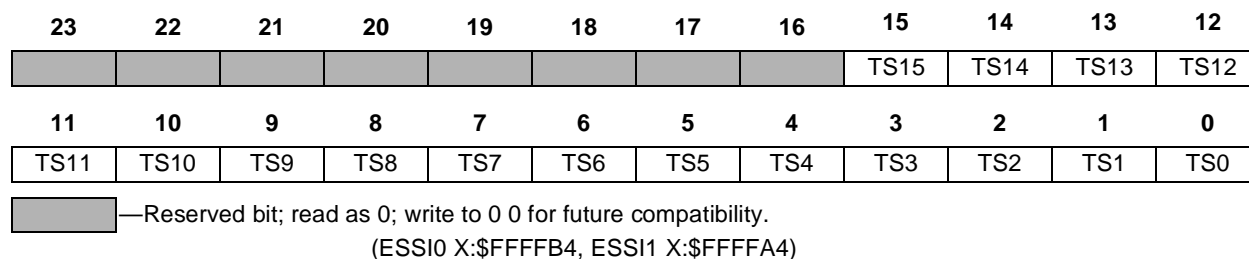
Figure 7-12. ESSI Transmit Slot Mask Register A (TSMA)
