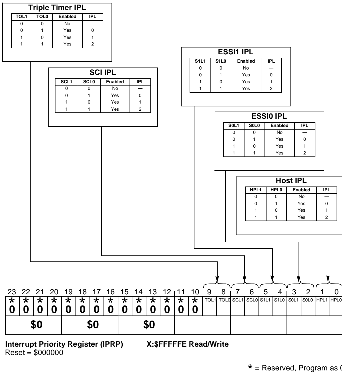
Figure B-4. Interrupt Priority Register Peripherals (IPRP)
