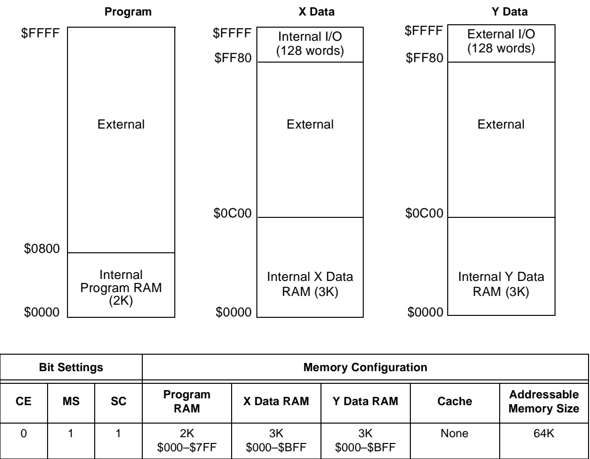
Figure 3-4. 16-Bit Space With Switched Program RAM (0, 1, 1)
