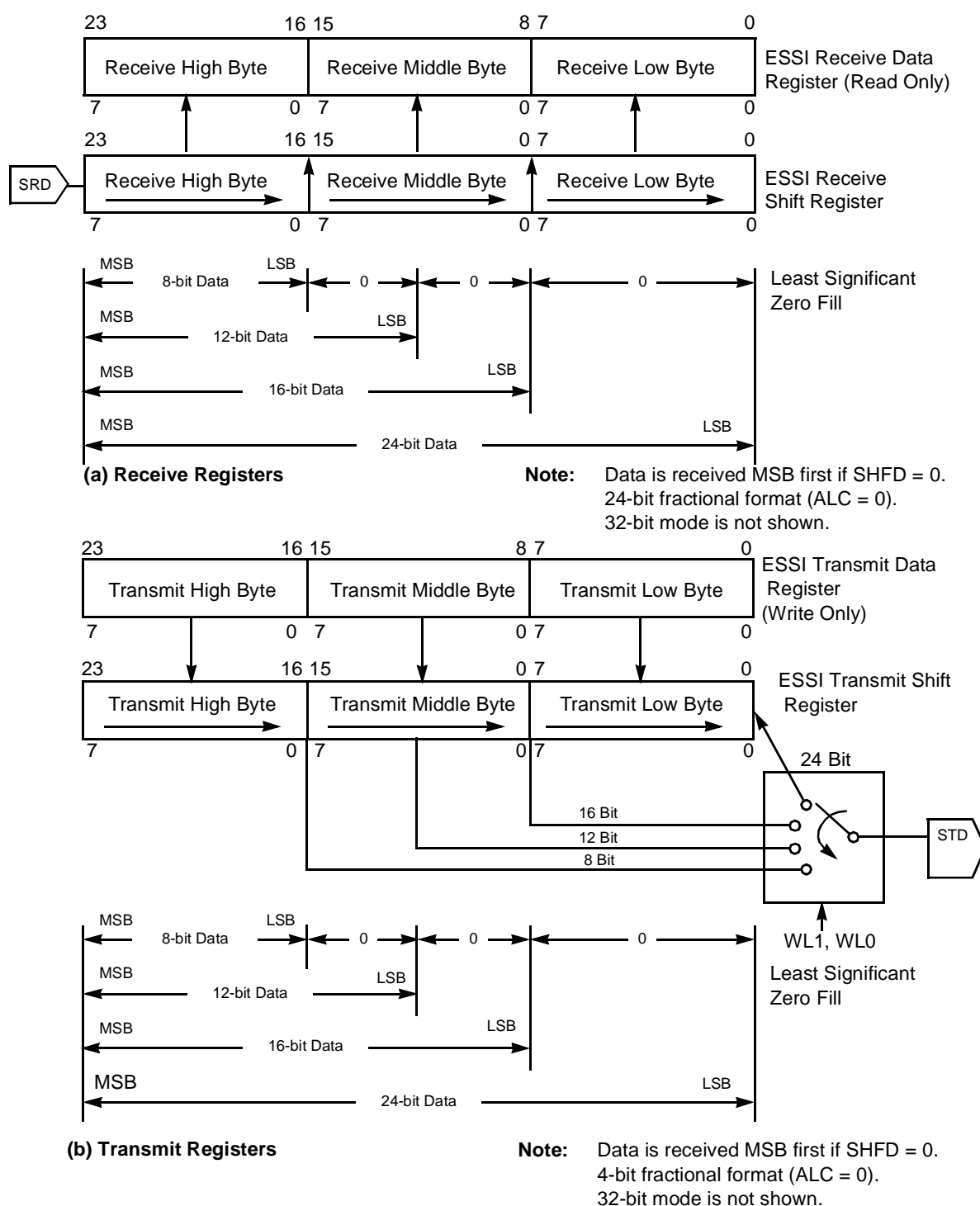
Figure 7-11. ESSI Data Path Programming Model (SHFD = 1)
