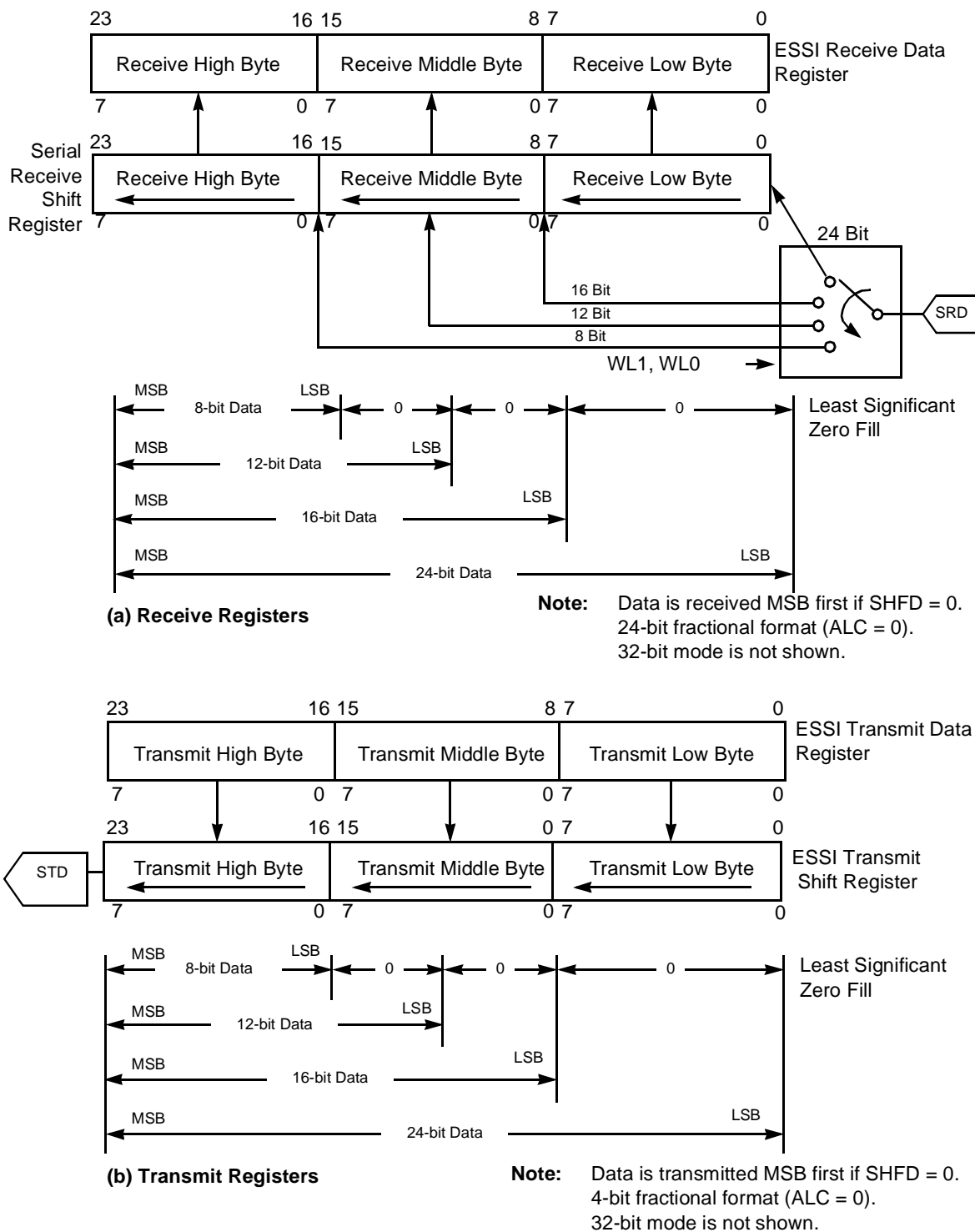
Figure 7-10. ESSI Data Path Programming Model (SHFD = 0)
