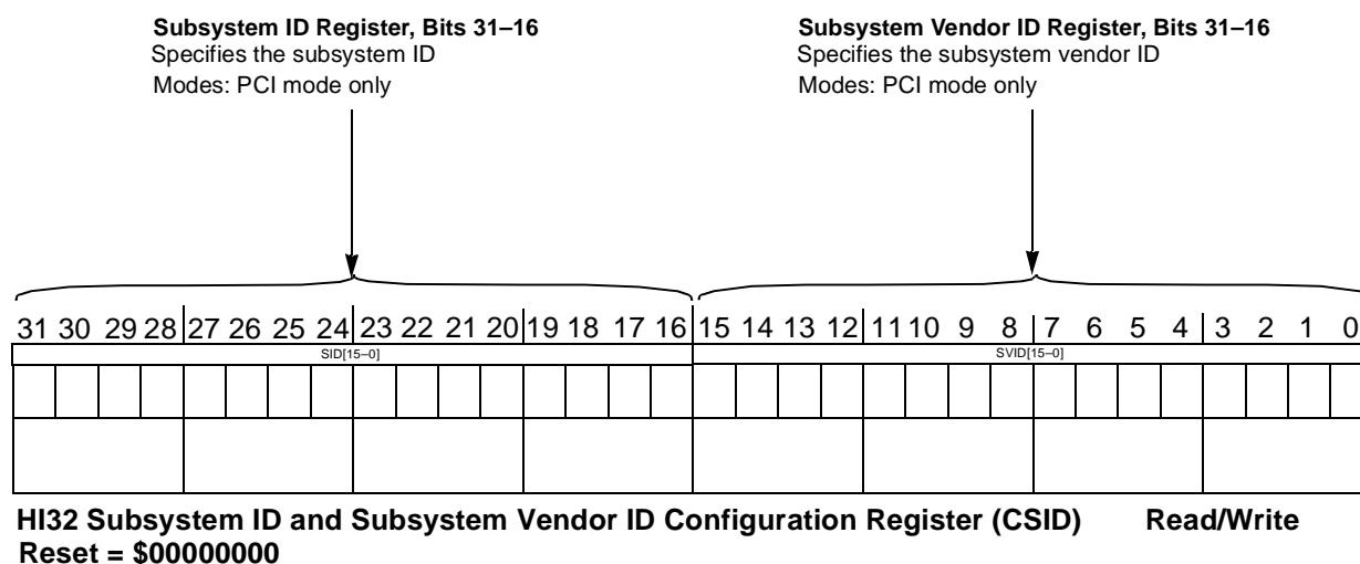
Figure B-19. Subsystem ID and Subsystem Vendor ID Configuration Register (CSID)
