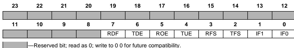
Figure 7-9. ESSI Status Register (SSISR)
