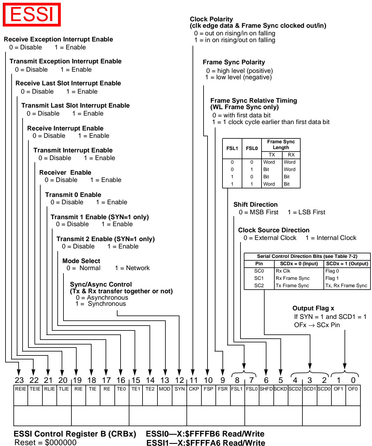
Figure B-21. ESSI Control Register B (CRB)
