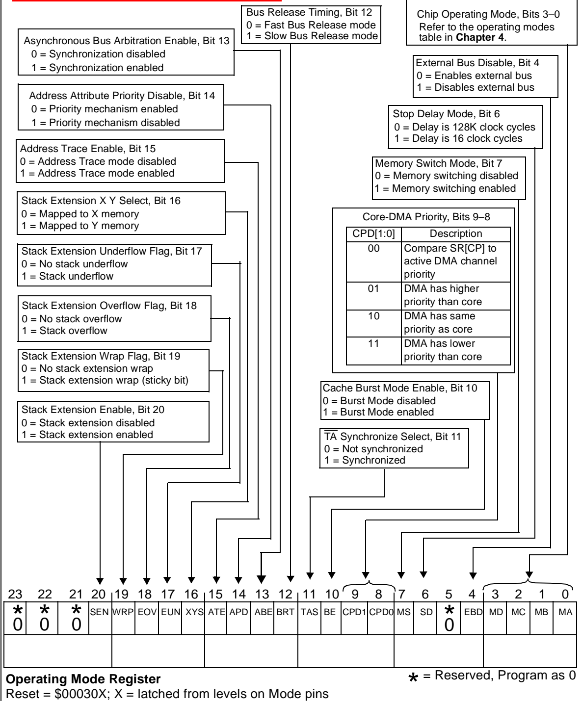
Figure B-2. Operating Mode Register (OMR)
