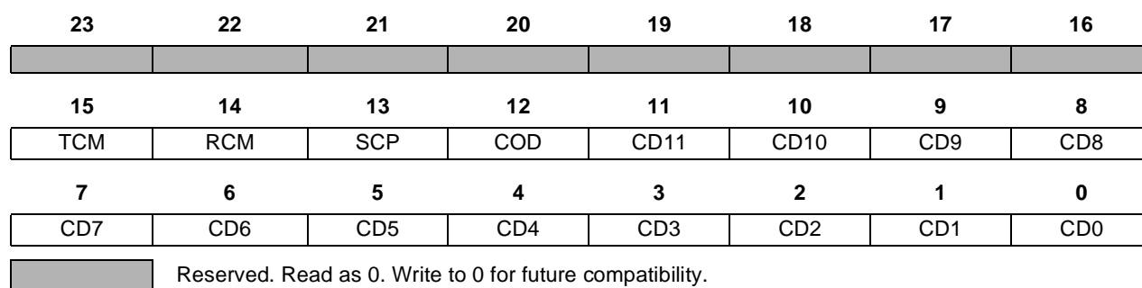
Figure 8-3. SCI Clock Control Register (SCCR)
