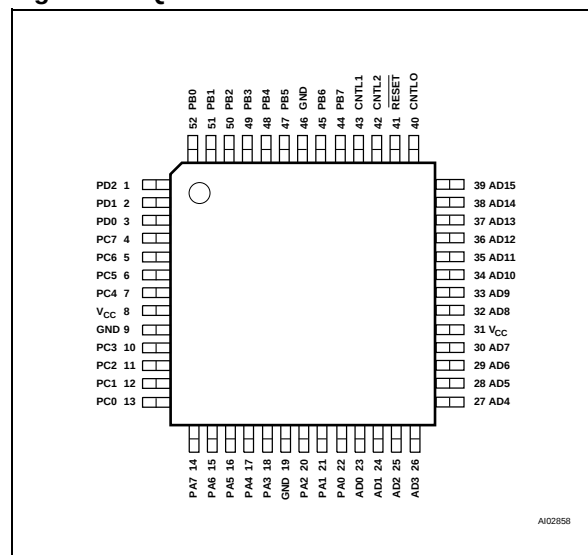
Figure 4. PQFP Connections
