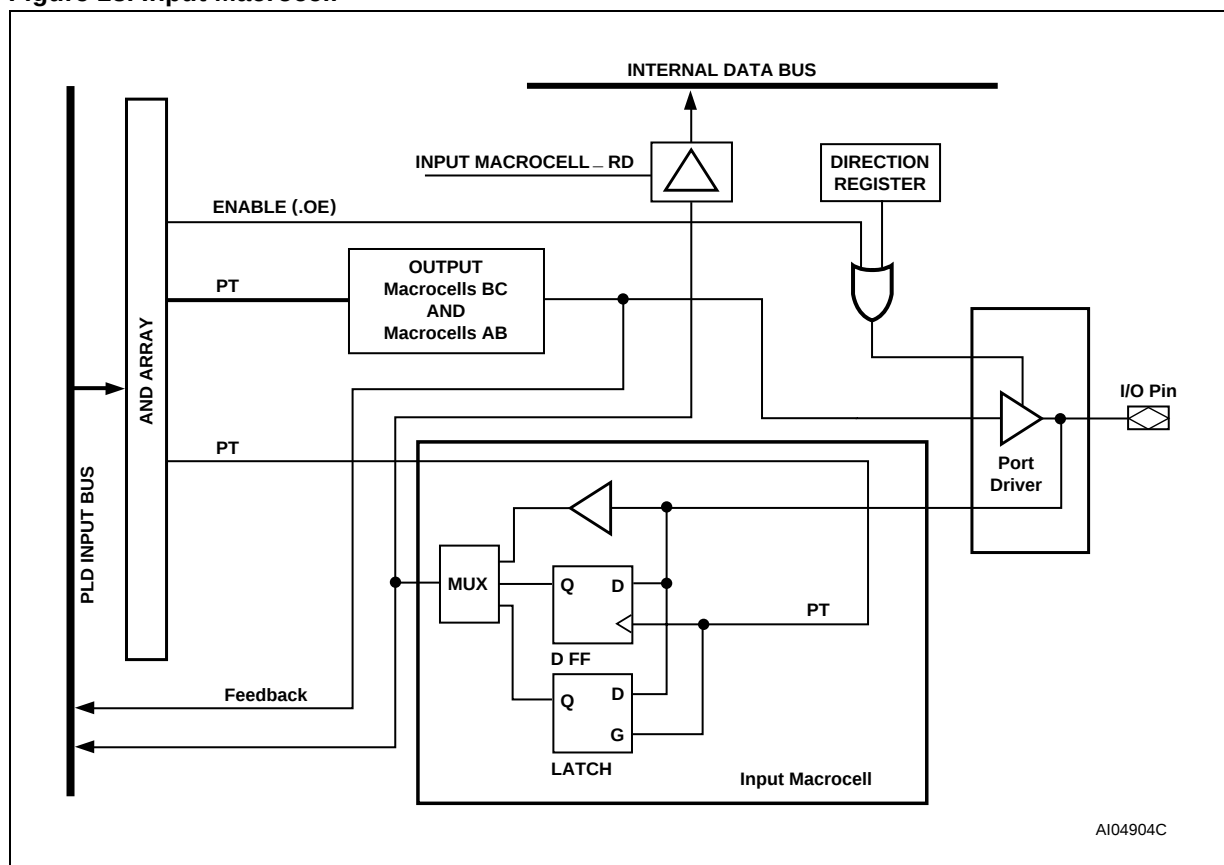
Figure 18. Input Macrocell
