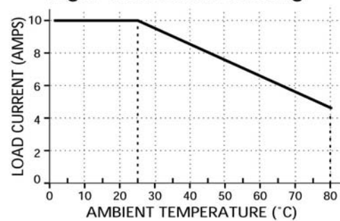
Fig.2 Forced Air Cooling
