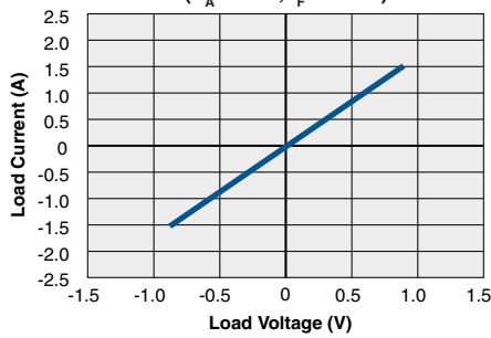
CPC1979 Typical Load Current vs. Load Voltage ( T_A = 25^\circ\text{C} , I_F = 10\text{mA} )
