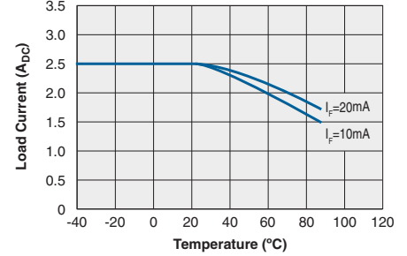
Typical Load Current vs. Temperature
