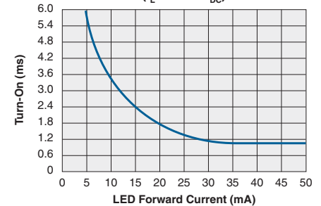
Typical Turn-On vs. LED Forward Current ( I_L=100\text{mA}_{\text{DC}} )
