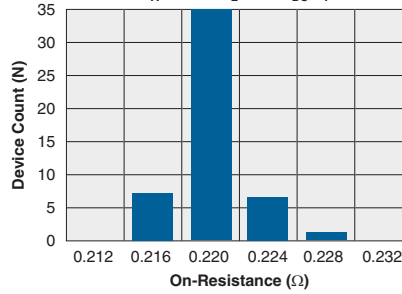
Typical On-Resistance Distribution (N=50, T_A=25^\circ\text{C} , I_L=1.0\text{A}_{\text{DC}} , I_F=10\text{mA} )
