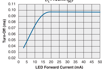
Typical Turn-Off vs. LED Forward Current ( I_L = 100\text{mA}_{\text{DC}} )
