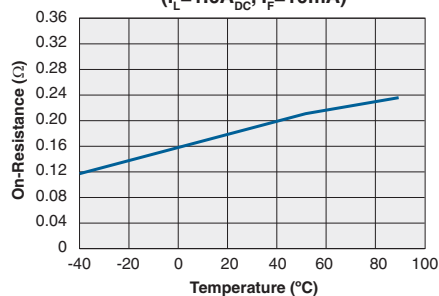
Typical On-Resistance vs. Temperature ( I_L = 1.0\text{A}_{\text{DC}} , I_F = 10\text{mA} )
