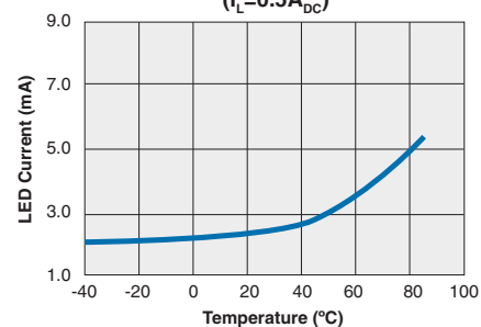
CPC1786 Typical I_F for Switch Operation vs. Temperature ( I_L = 0.5A_{DC} )
