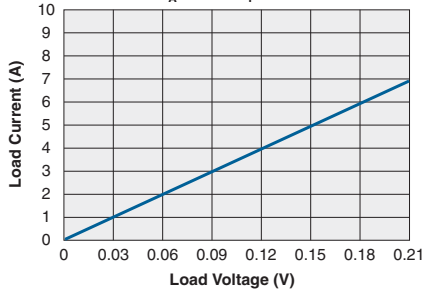
CPC1718 Typical Load Current vs. Load Voltage ( T_A = 25^\circ\text{C} , I_F = 10\text{mA} )
