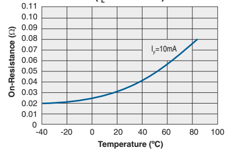
CPC1718 Typical On-Resistance vs. Temperature ( I_L = \text{Max Rated} )
