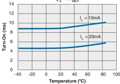
CPC1708 Typical Turn-On vs. Temperature ( I_L=1A_{DC} )
