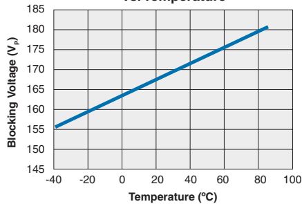
CPC1708 Blocking Voltage vs. Temperature
