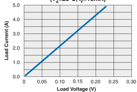
CPC1708 Typical Load Current vs. Load Voltage ( T_A = 25°C , I_F = 10mA )
