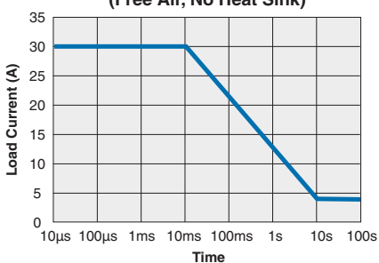
CPC1708 Energy Rating Curve (Free Air, No Heat Sink)
