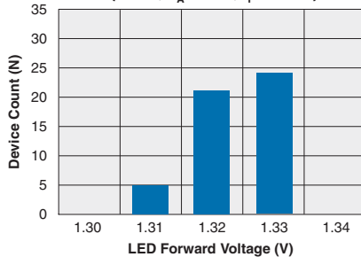
CPC1708 Typical LED Forward Voltage Drop (N=50, T_A=25^\circ\text{C} , I_F=10\text{mA} )
