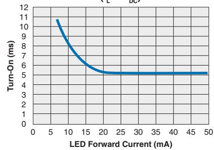
CPC1708 Typical Turn-On vs. LED Forward Current ( I_L=1A_{DC} )
