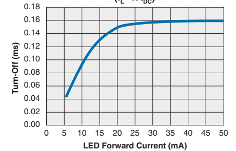
CPC1708 Typical Turn-Off vs. LED Forward Current ( I_L=1A_{DC} )
