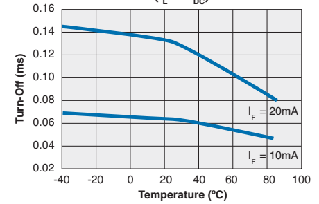
CPC1708 Typical Turn-Off vs. Temperature ( I_L=1A_{DC} )
