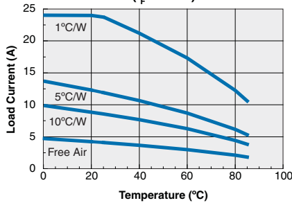
CPC1708 Typical Maximum Load Current vs. Temperature with Heat Sink ( I_F=20\text{mA} )
