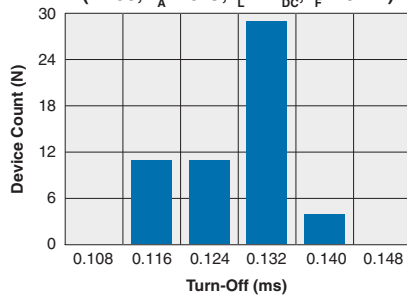
CPC1708 Typical Turn-Off Time (N=50, T_A=25^\circ\text{C} , I_L=1A_{DC} , I_F=20\text{mA} )
