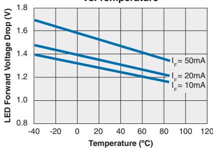
CPC1708 Typical LED Forward Voltage Drop vs. Temperature
