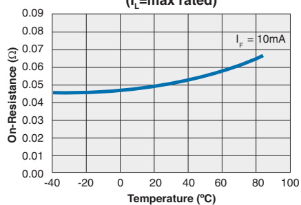
CPC1708 Typical On-Resistance vs. Temperature ( I_L = \text{max rated} )
