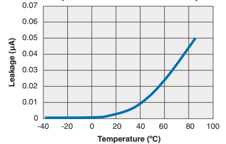
CPC1708 Typical Leakage vs. Temperature at Maximum Rated Voltage (Measured Across Pins 1 & 2)
