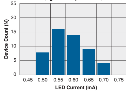
CPC1225N Typical IF For Switch Operation ( T_A=25^\circ\text{C} , I_L=120\text{mA} )
