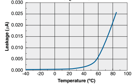
CPC1225N Typical Leakage vs. Temperature (Measured Across Pins 3 & 4) ( V_L=400\text{V} )
