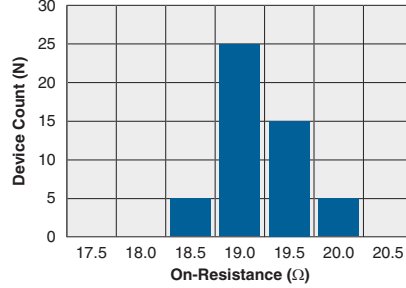
CPC1225N Typical On-Resistance Distribution ( T_A=25^\circ\text{C} , I_L=120\text{mA} , I_F=2\text{mA} )
