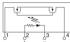
CPC1218 Pinout
