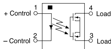
CPC1025N Pinout
