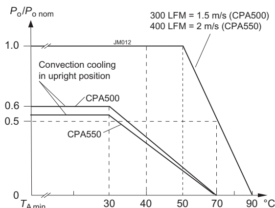
Fig. 4c Output power versus temperature T_A at V_{i\text{ nom}} (CPA500/550)
