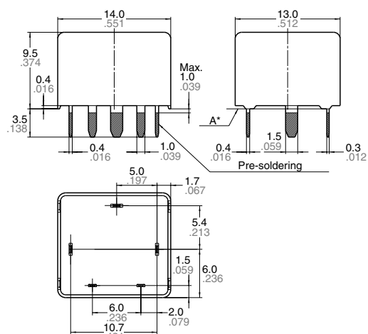
External dimensions
