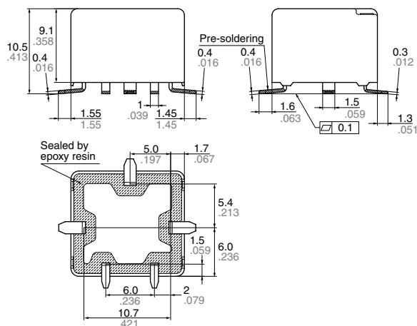
External dimensions
