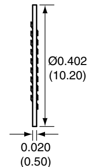
WASHER
