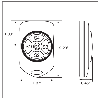
Figure 1: Package Dimensions
