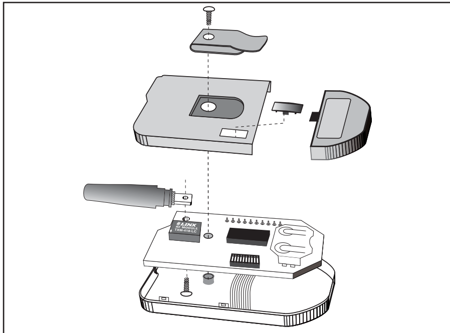
Figure 5: CMD-HHLR-*** Assembly
