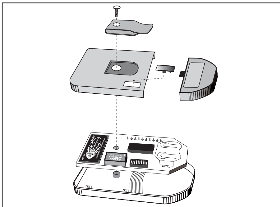
Figure 5: CMD-HHCP-*** Assembly
