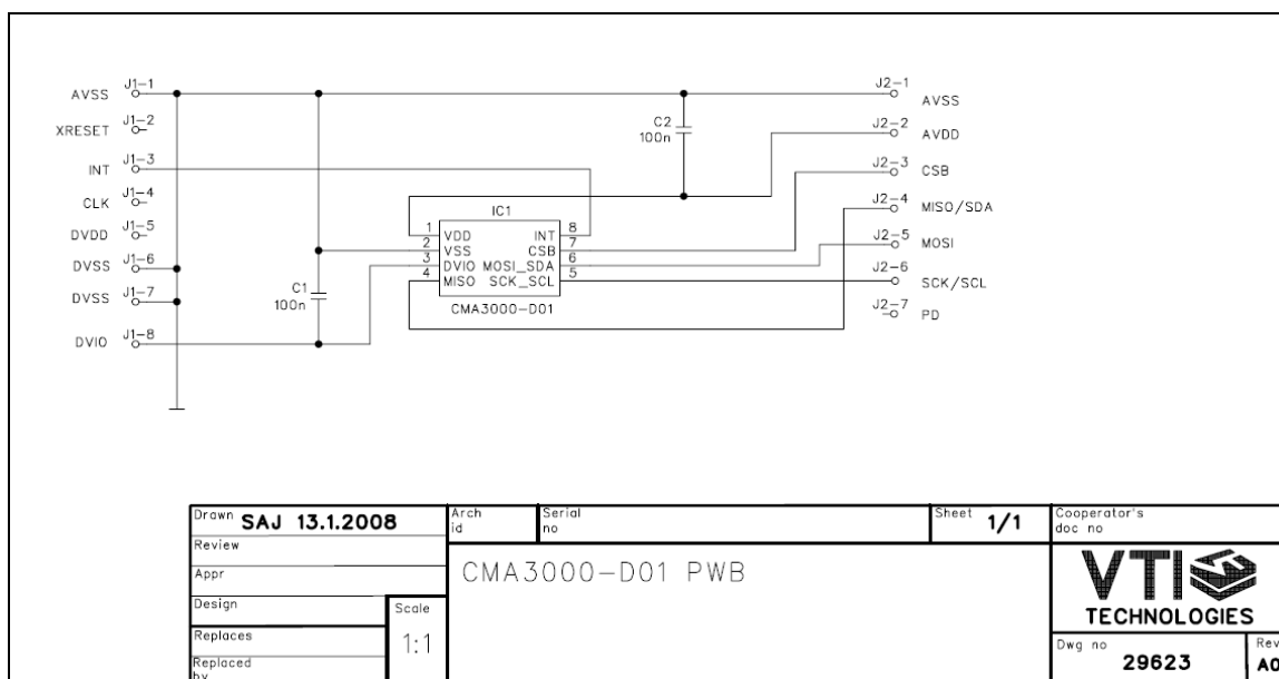
Figure 1. CMA3000-D0X PWB circuit diagram.
