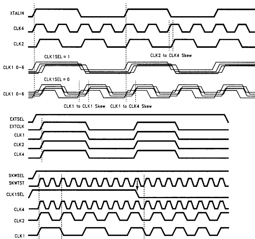
FIGURE 1. Waveforms
