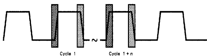
FIGURE 2. Jitter
