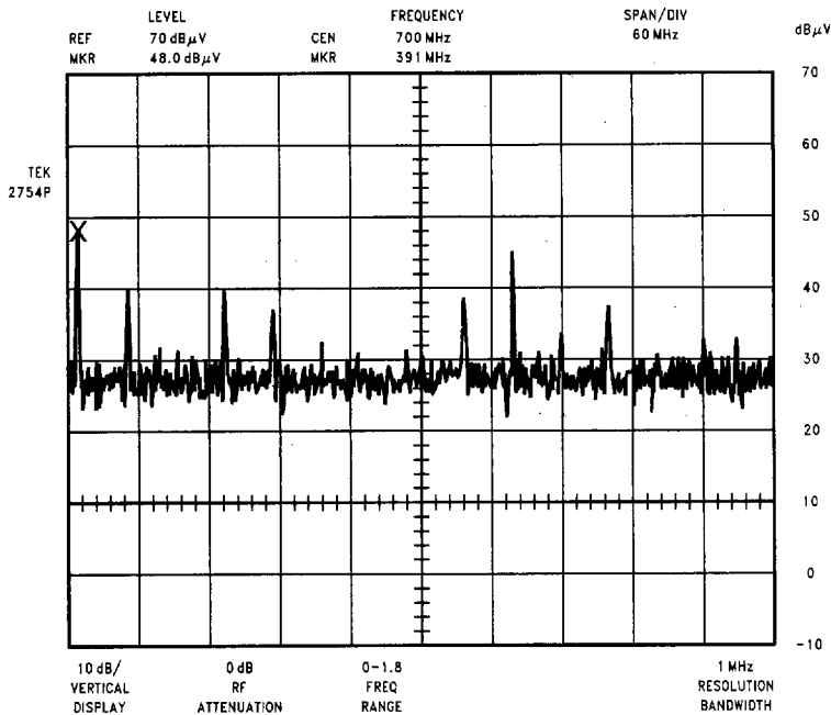
FIGURE 5. CGS702
