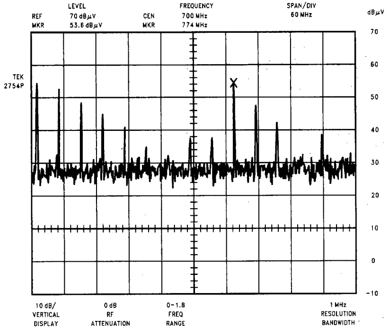
FIGURE 4. CGS700
