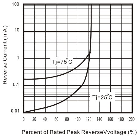
Fig. 1 - Reverse Characteristics
