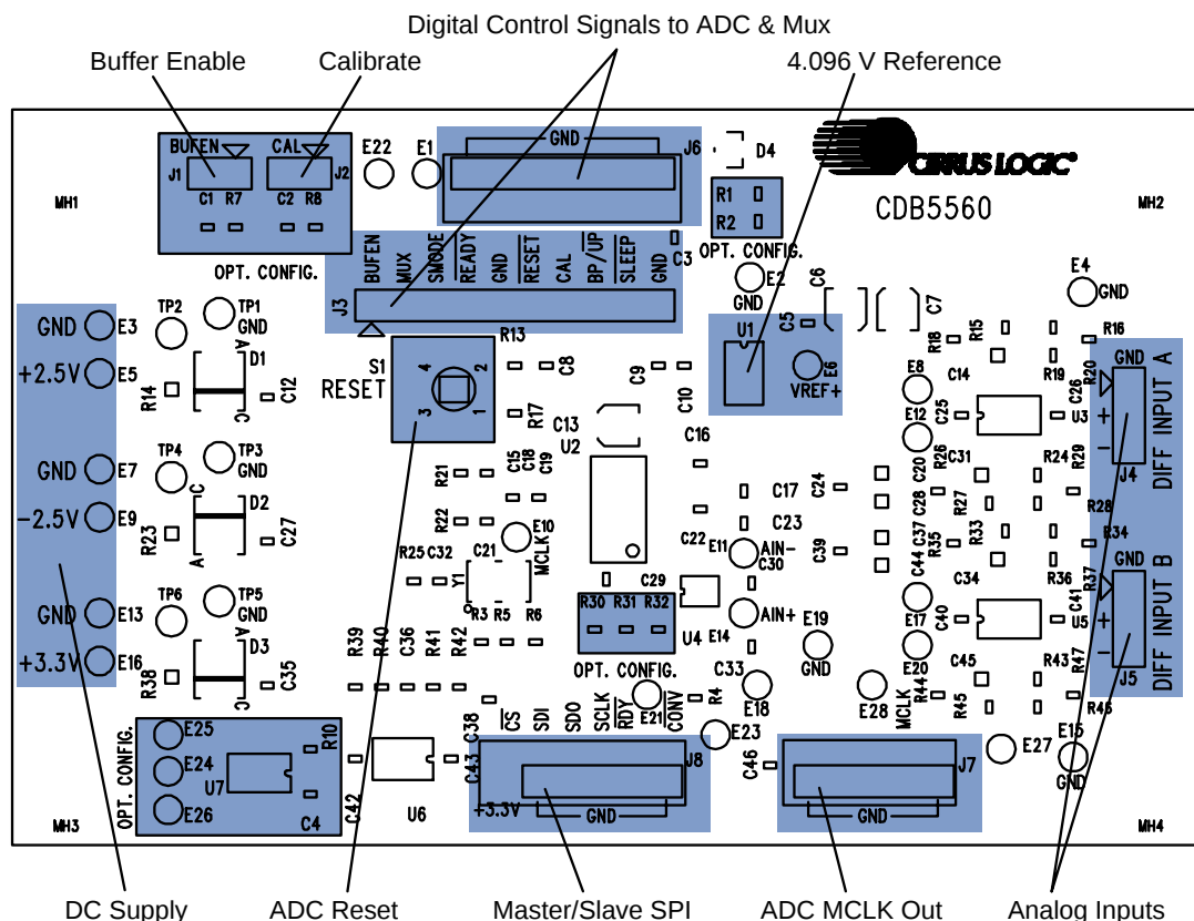
Figure 2. CDB5560 Board Layout
