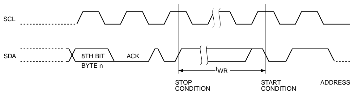
Figure 3. Start/Stop Timing
