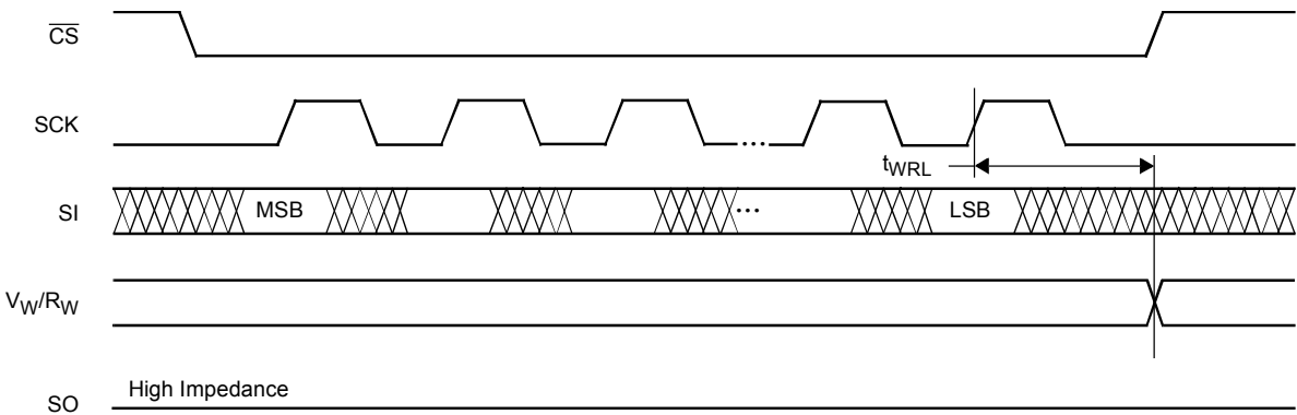
Figure 3. Potentiometer Timing (for All Load Instructions)
