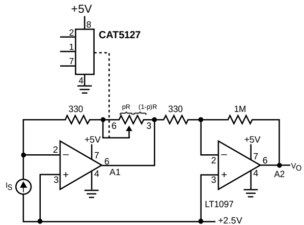
Programmable I to V convertor
