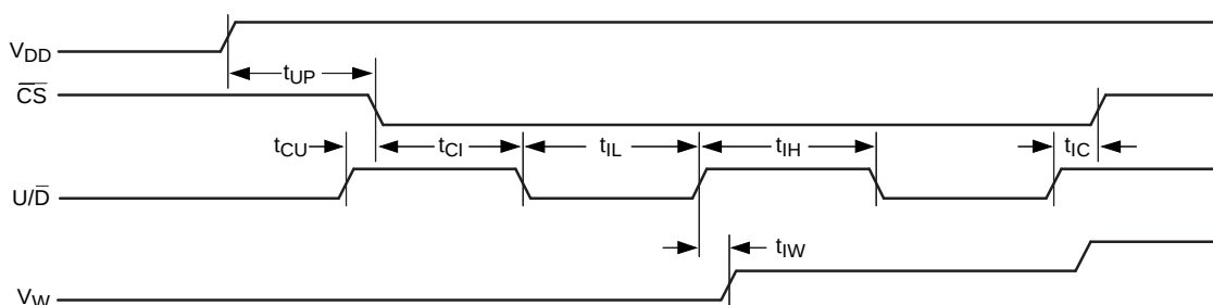
Figure 1. Increment Mode Serial Interface Timing Diagram
