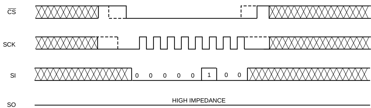
Figure 3. WRDI Timing
