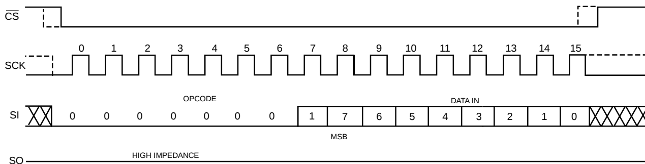
Figure 8. WRSR Timing
