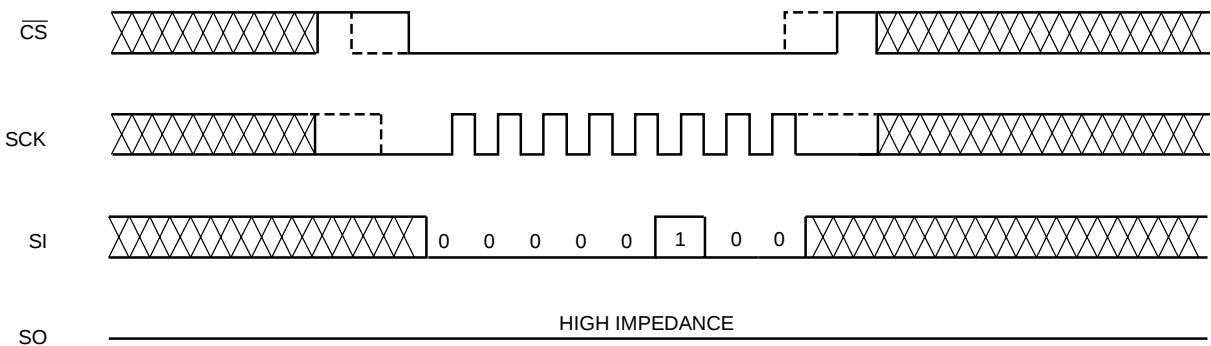
Figure 5. WRDI Timing
