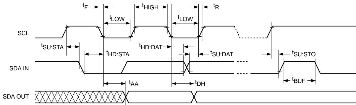
Figure 6. Bus Timing
