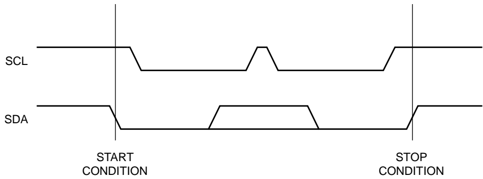
Figure 3. START/STOP Conditions
