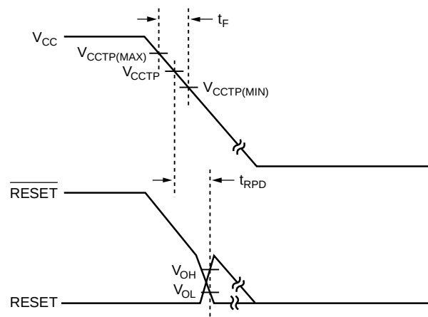
Figure 2. Timing Diagram: Power Down
