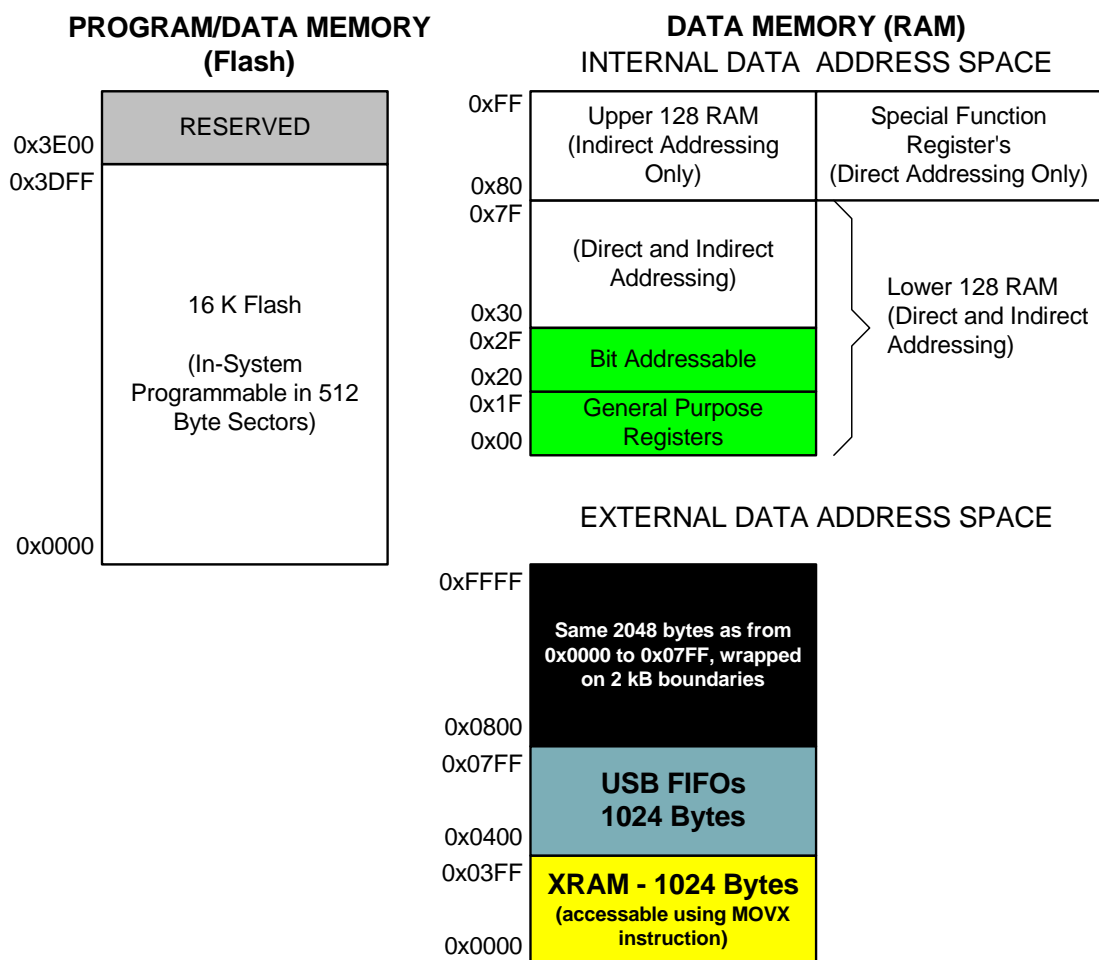
Figure 9.2. Memory Map
