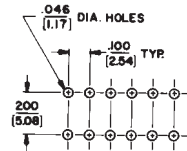
RECOMMENDED PC BOARD LAYOUT (Component Side)
