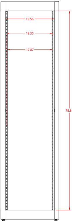
FRONT VIEW
