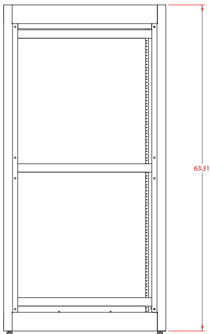
L.S. VIEW
