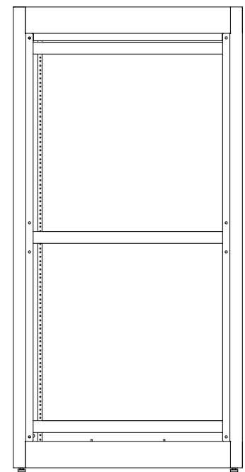
R.S. VIEW
