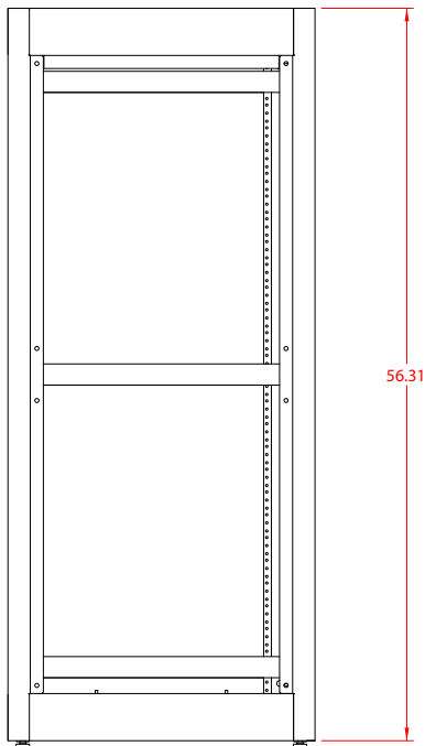
L.S. VIEW
