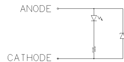
LED CIRCUIT
