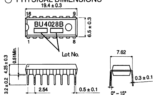
BU4028(DIP16)(UNIT:[mm])
