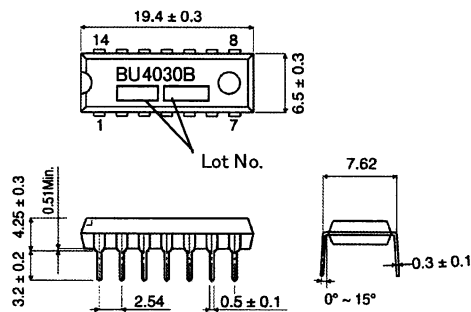
BU4030B(DIP14)(UNIT:[mm])
