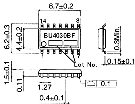
BU4030BF(SOP14)(UNIT:[mm])
