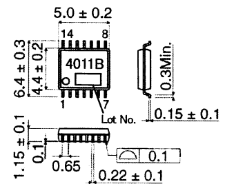
BU4011BFV(SSOP-B14)( UNIT:[mm])
