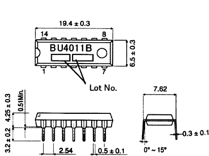
BU4011B(DIP14)(UNIT:[mm])
