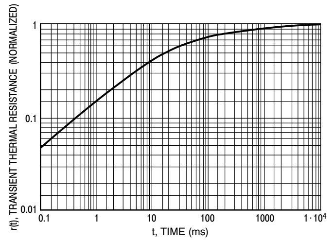
Figure 4. Thermal Response
