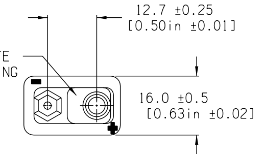
TOP VIEW OF BATTERY
