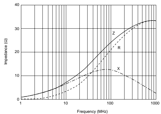
BLM21PG220SN1
