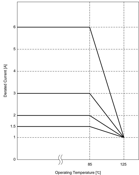
Derating
