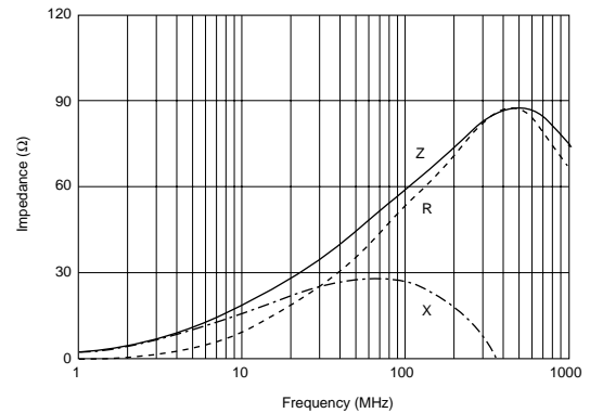
BLM21PG600SN1
