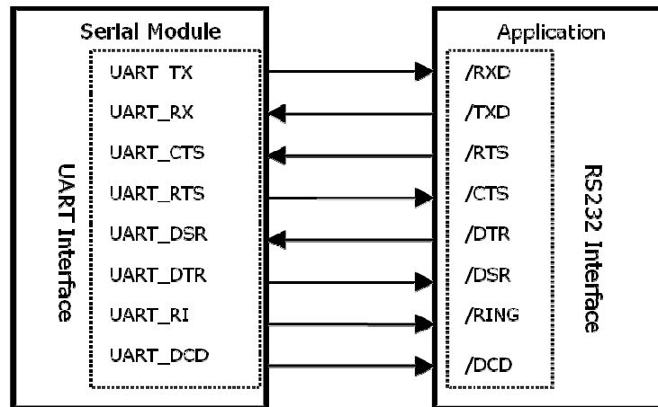
Figure 6.1 : UART interfaces
