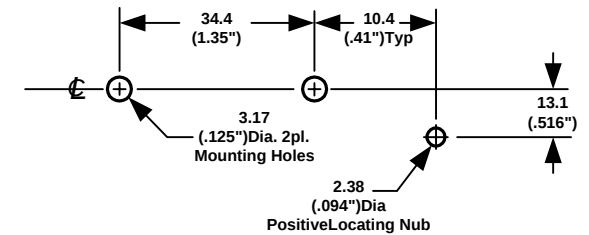
Standard Pc Version P.C. Board Hole layout
