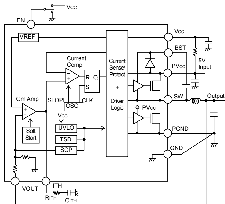
Fig.2 BD9134MUV Block Diagram
