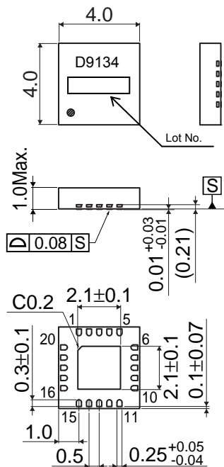
Fig.1 BD9134MUV TOP View
