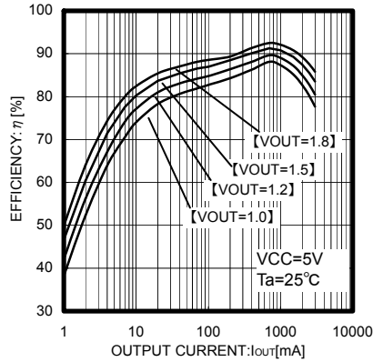
Fig.7 Efficiency
