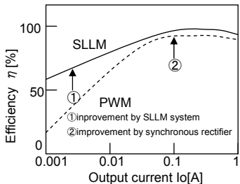
Fig.19 Efficiency
