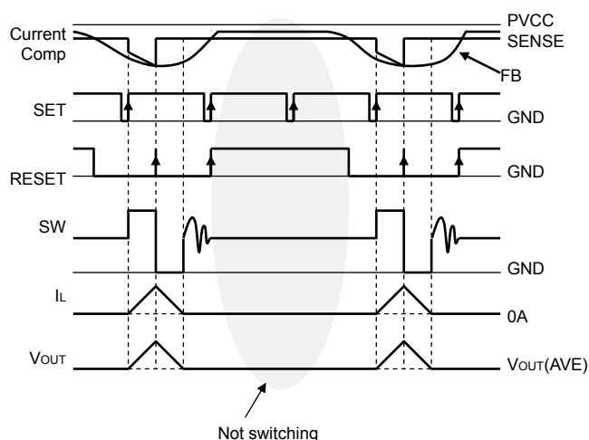
Fig.23 SLLM TM switching timing chart
