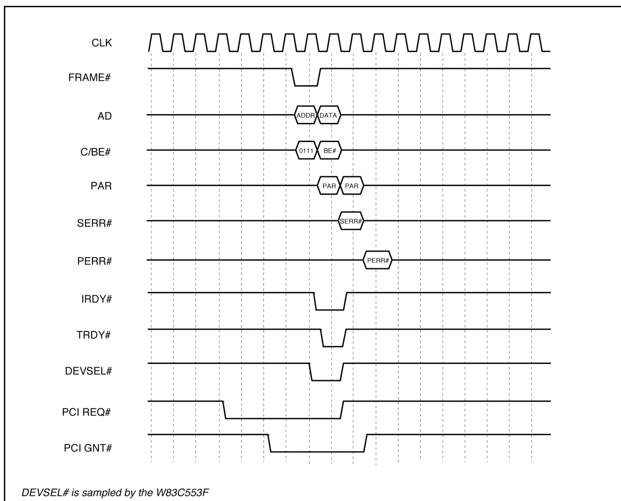
Figure 3-7. Master Memory Write Timing
